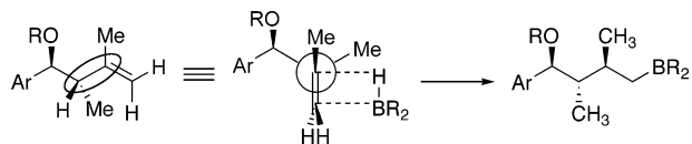
FIGURE 3. A^{1,3} -strain model for diastereofacial selectivity.
