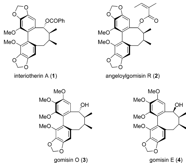
FIGURE 2. Dibenzocyclooctadiene natural product targets.
