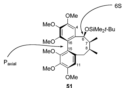
FIGURE 4. Relative configuration of biaryl coupled product 51 .
