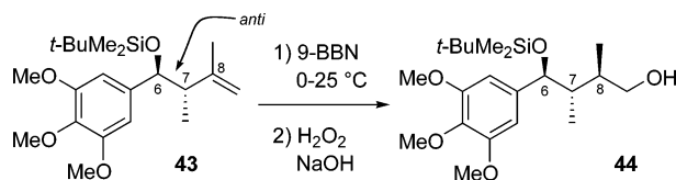
FIGURE 3. A^{1,3} -strain model for diastereofacial selectivity.
