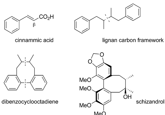
FIGURE 1. Biosynthetic considerations in the lignan family of plant natural products.
